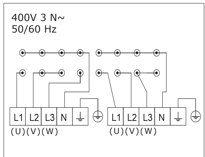
Connection diagram for Eterno sauna heater – 12.0 kW (dual-circuit) with PE
