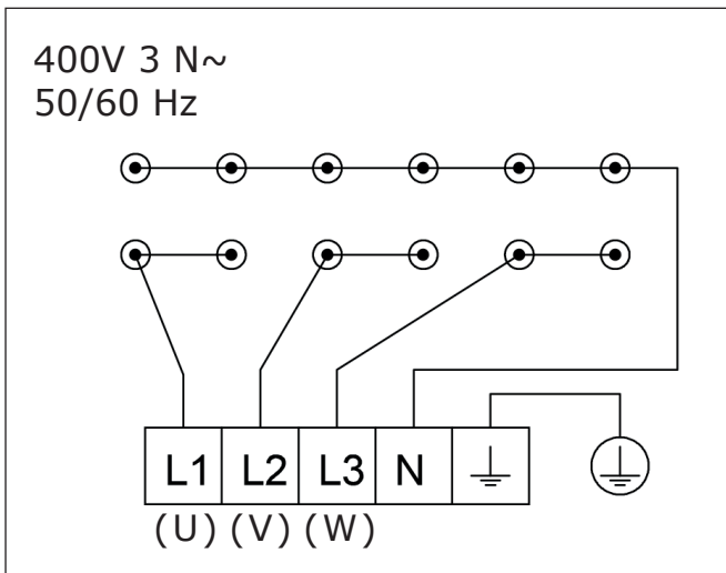
Connection diagram for Eterno sauna heater – 9.0 kW and 10.5 kW models
