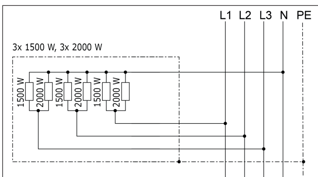
Sauna heater Eterno with 10.5 kW
