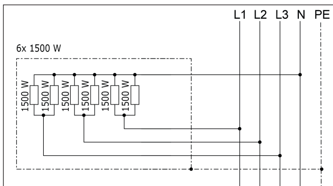
Sauna heater Eterno with 9.0 kW
