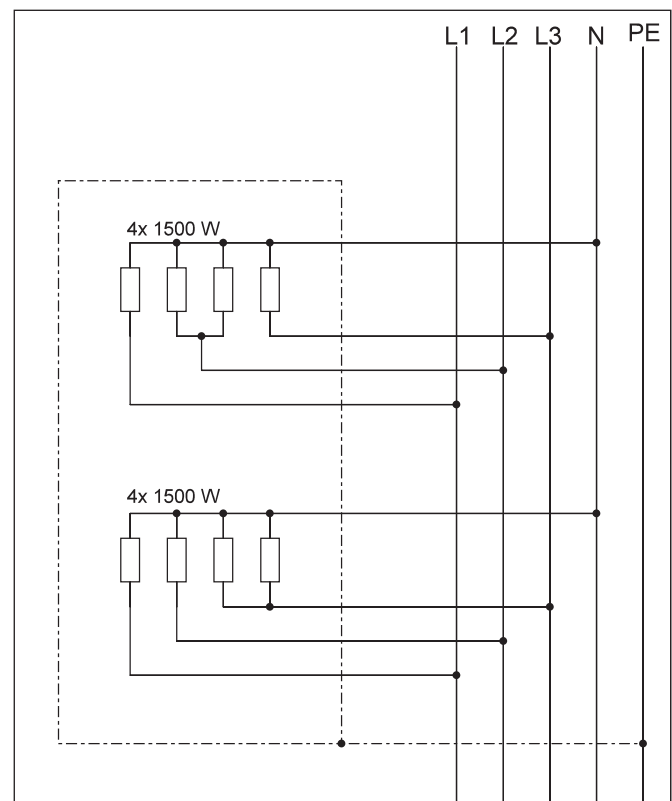
Sauna heater Eterno with 12.0 kW (dual-circuit)
